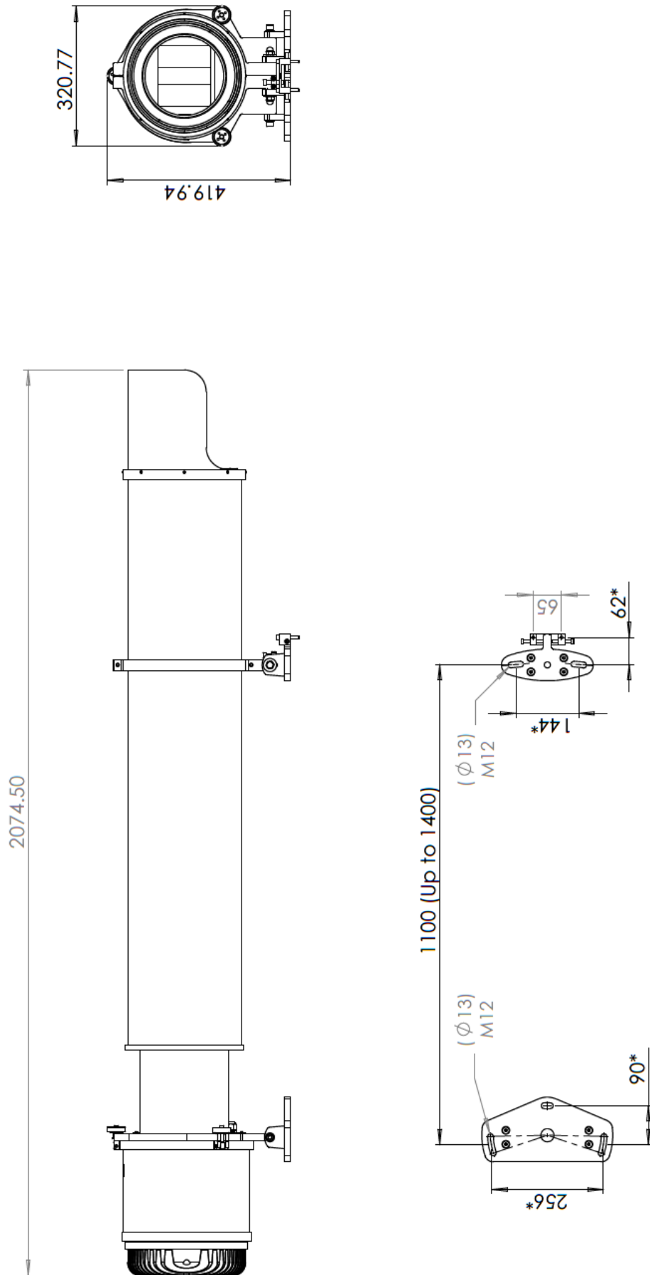
PEL-7 5D General Assembly Drawing
