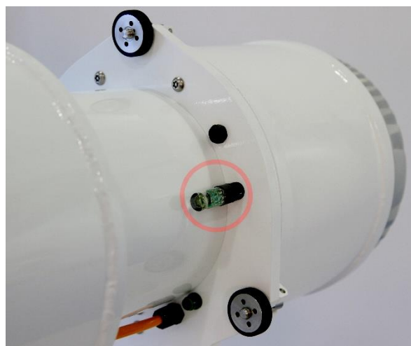
Location of the PEL-7 Programming Infrared Receiver and Daylight Detector
