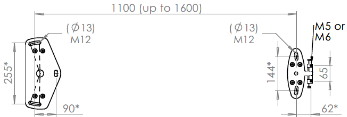
PEL-7 3.5D Model's Mounting Brackets – Plan View
