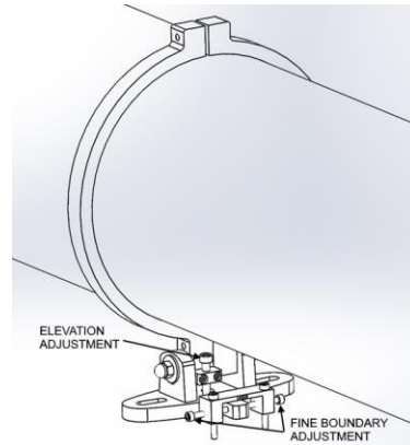
PEL-7 3.5D Model's Alignment Mechanism
