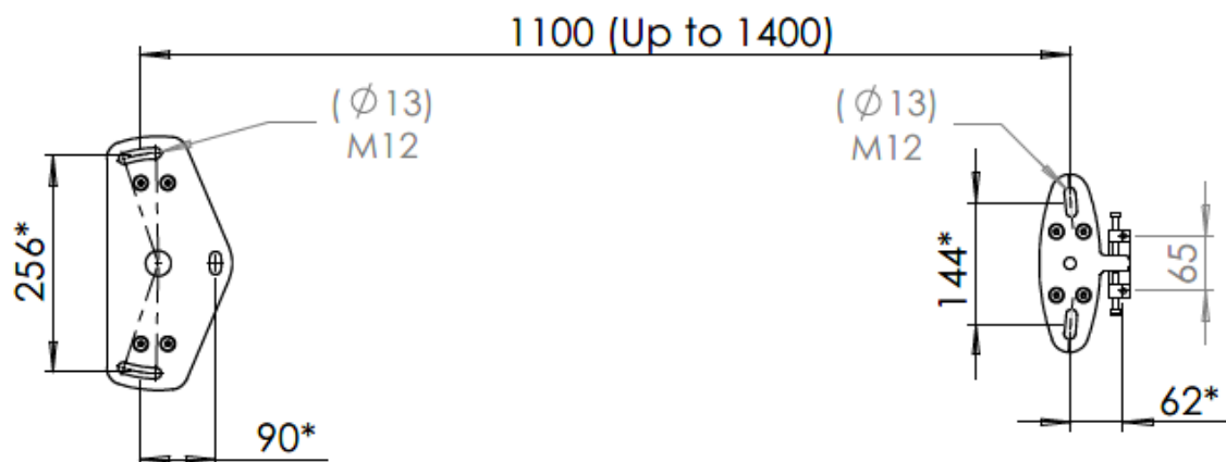
PEL-7 5D Model's Mounting Brackets – Plan View
