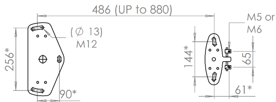
PEL-7 10D Model's Mounting Brackets – Plan View
